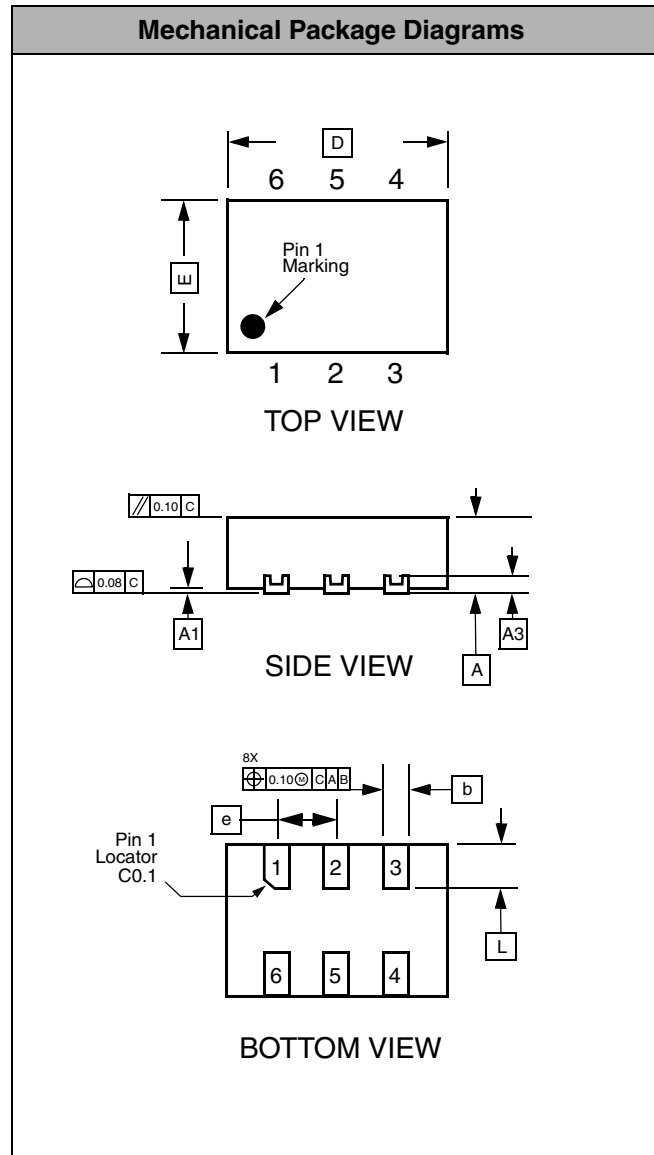
Dimensions for 6-Lead, 0.5mm pitch superDFN-0.5 package
