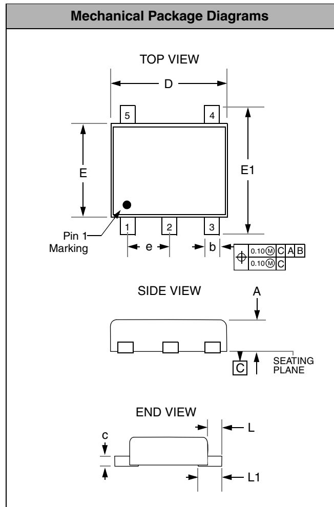
Package Dimensions for SOT-953
