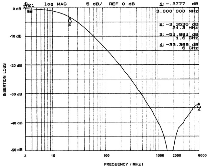
Figure 1. Typical EMI Filter Performance (0VDC, 50 Ohm Environment)
