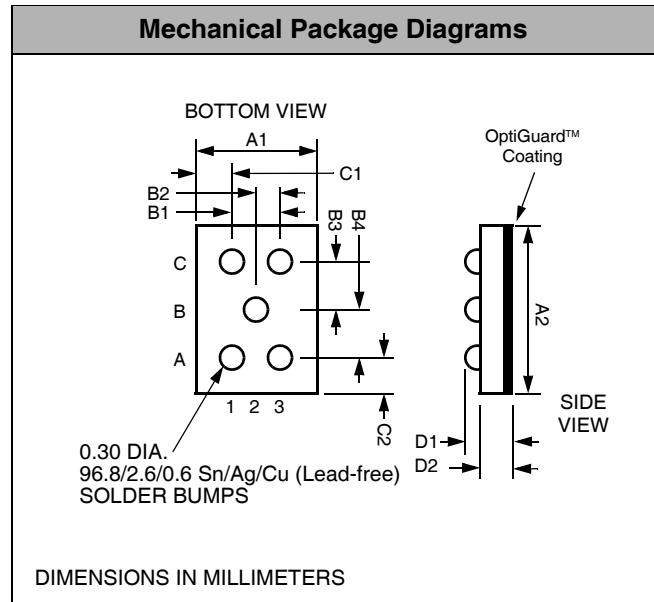
Package Dimensions for CM1416 Chip Scale Package
